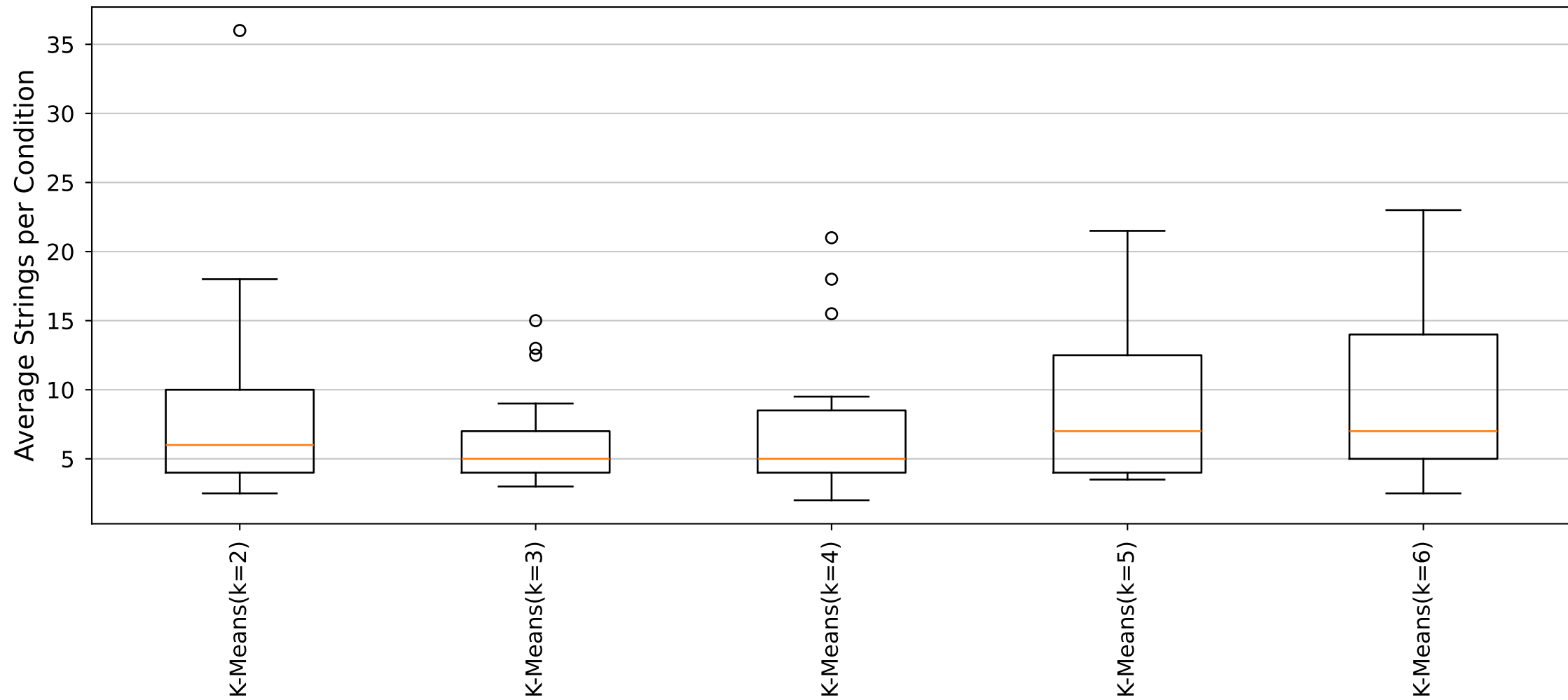
YARA Rules Average Strings per Condition Distribution (Cluster24_Size6 dataset)
